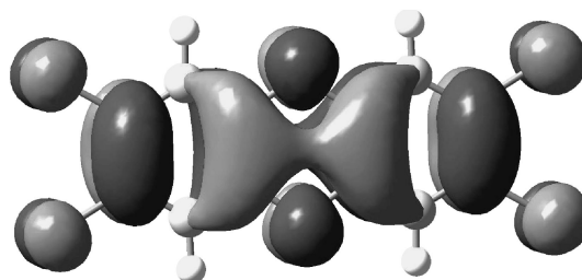
Figure 2. HOMO of 2,3,7,8-tetrachlorinated dibenzo- p -dioxin (2,3,7,8-T 4 CDD) (#48).
